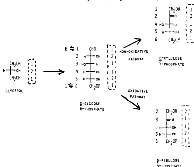
Scheme VIII. Predicted Derivation of the Carbon Atoms of a Pentose from the Carbon Atoms of Glucose (Plain Numbers) and from the Carbon Atoms of Glycerol (Ringed Numbers)
