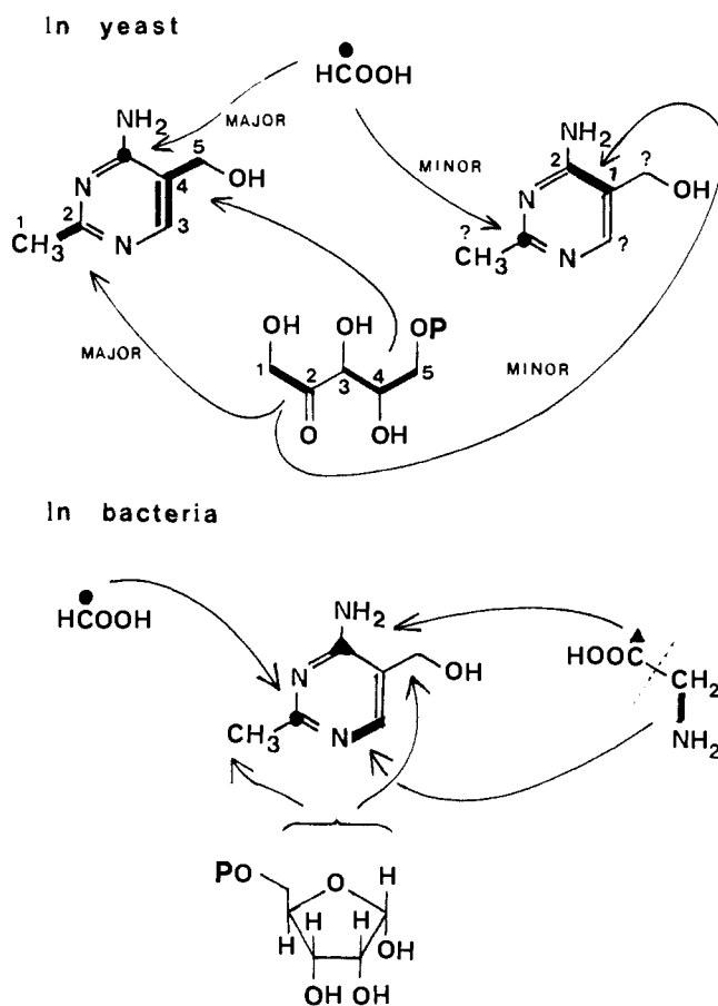
Scheme IX. Biosynthesis of the Pyrimidine Unit of Thiamin in Yeast and in Bacteria. Presursor-Product Relationships (Numbers Refer to the Carbon Atoms of a Pentose, Throughout)
