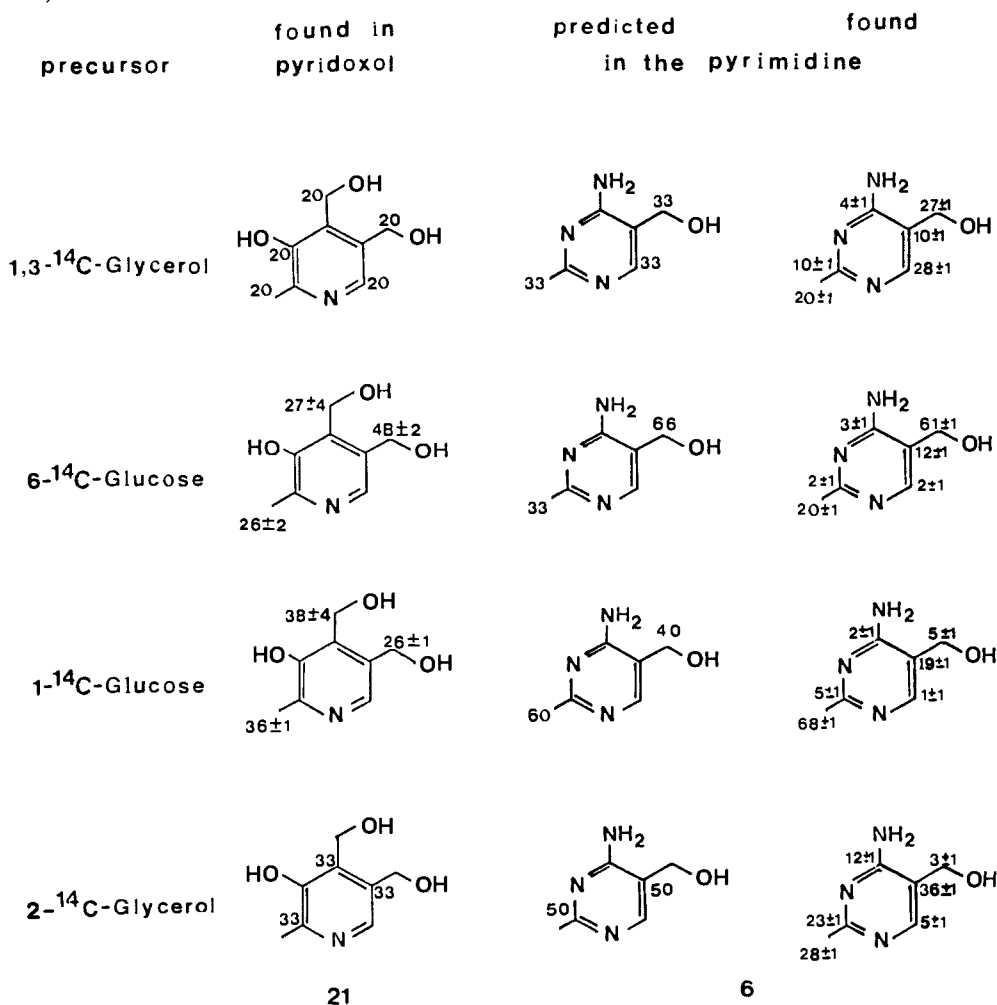
Scheme VI. Distribution of Label from Glucose and Glycerol, Observed in Pyridoxol, Compared with That Predicted and That Actually Observed within the Pyrimidine Unit of Thiamin (Numbers Represent Percent of the Total Activity of the Intact Molecule within the Indicated Carbon Atom)
