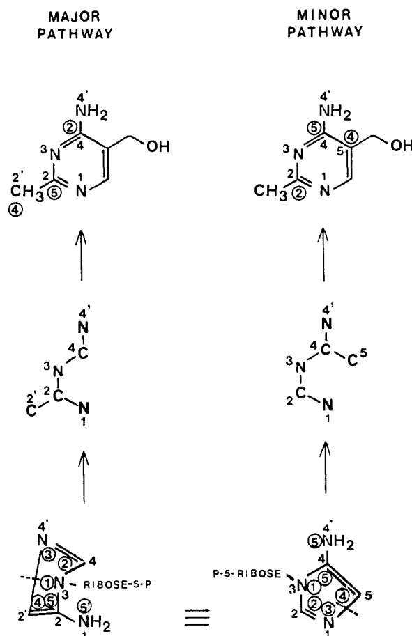
Scheme X. Biogenetic Anatomy of the Pyrimidine Unit of Thiamin a
